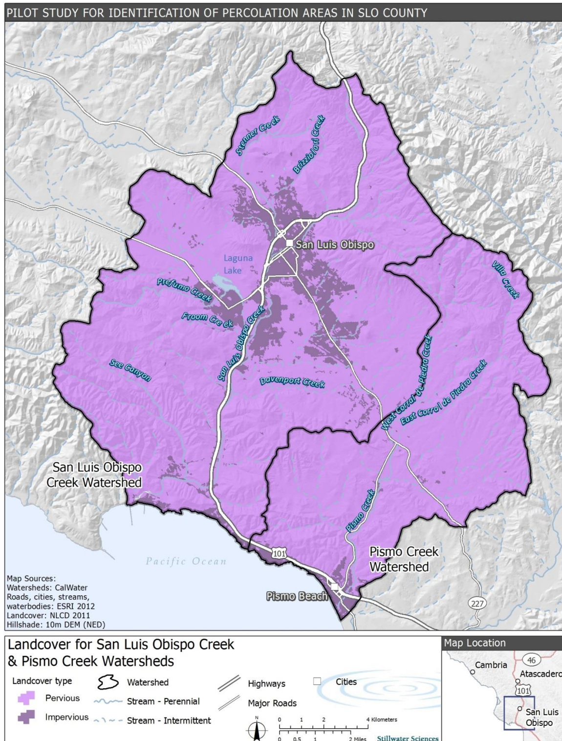
Figure 12. Generalized landcover classes used for the PLU analysis in the San Luis Obispo Creek and Pismo Creek watersheds.
