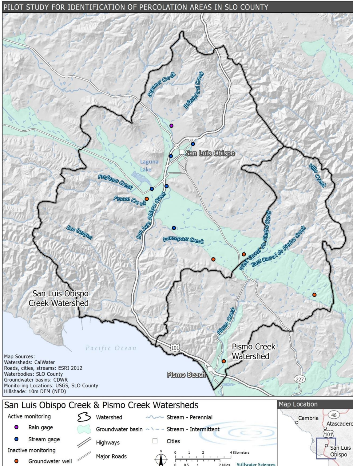
Figure 4. Hydrography, wells, and hydrologic monitoring stations in the San Luis Obispo Creek and Pismo Creek watersheds.
