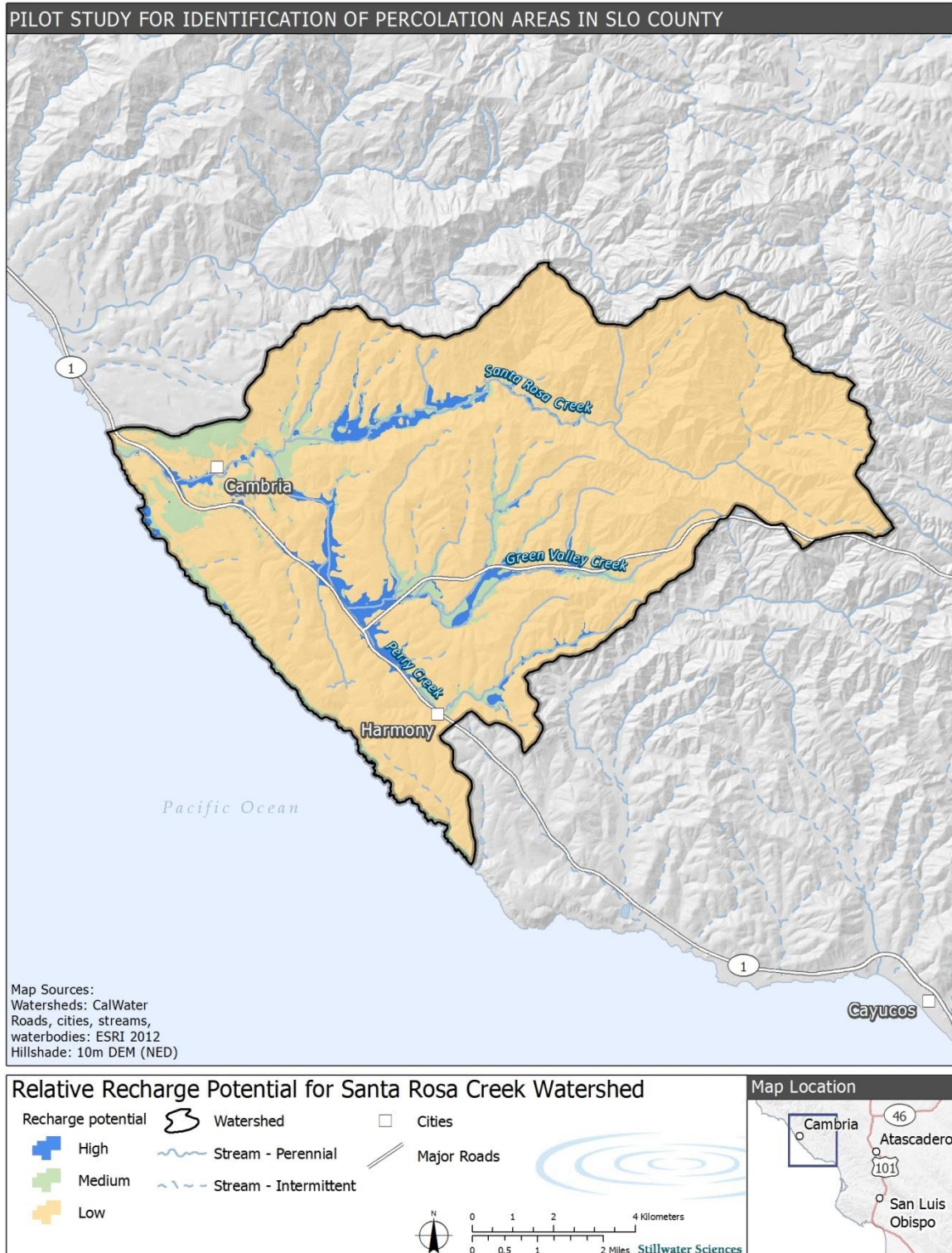
Figure 16. Predicted relative potential of intrinsic percolation in the Santa Rosa Creek watershed.
