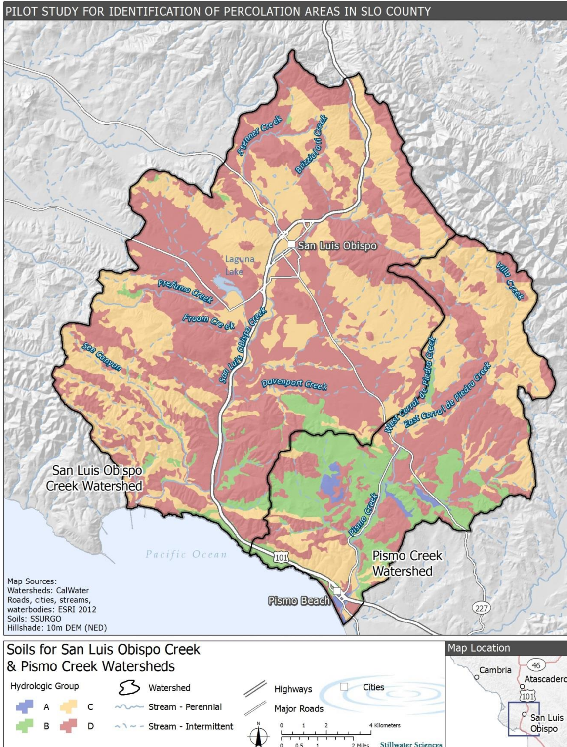
Figure 11. Generalized soil classes used for the PLU analysis in the San Luis Obispo Creek and Pismo Creek watersheds.
