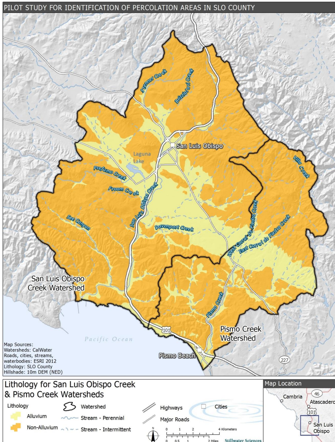
Figure 10. Generalized lithology classes used for the PLU analysis in the San Luis Obispo Creek and Pismo Creek watersheds.
